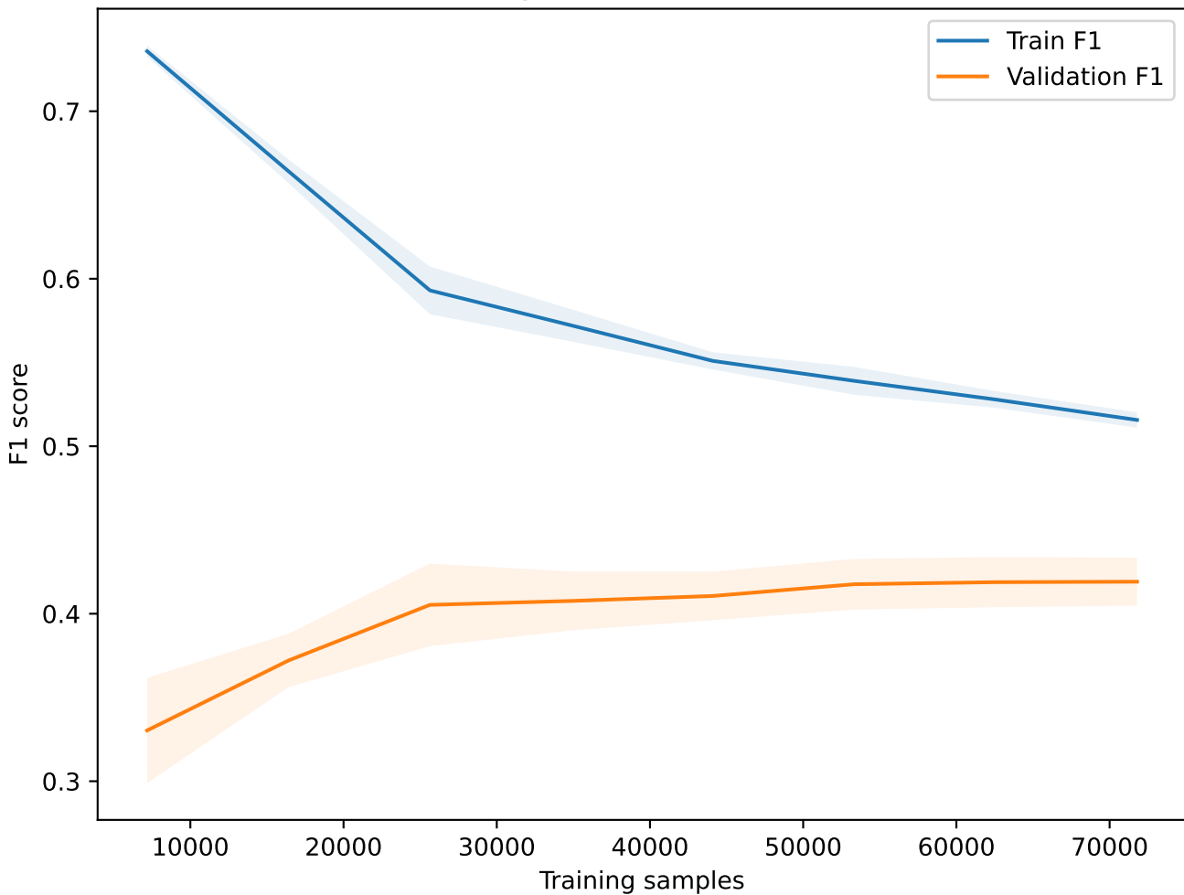
Learning curve - Random Forest
